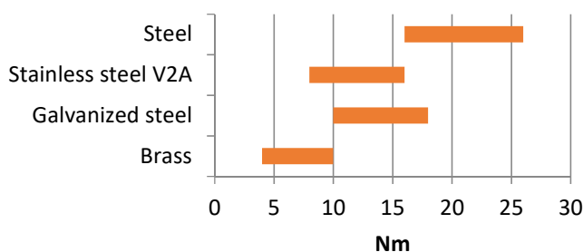
Breakloose torque
